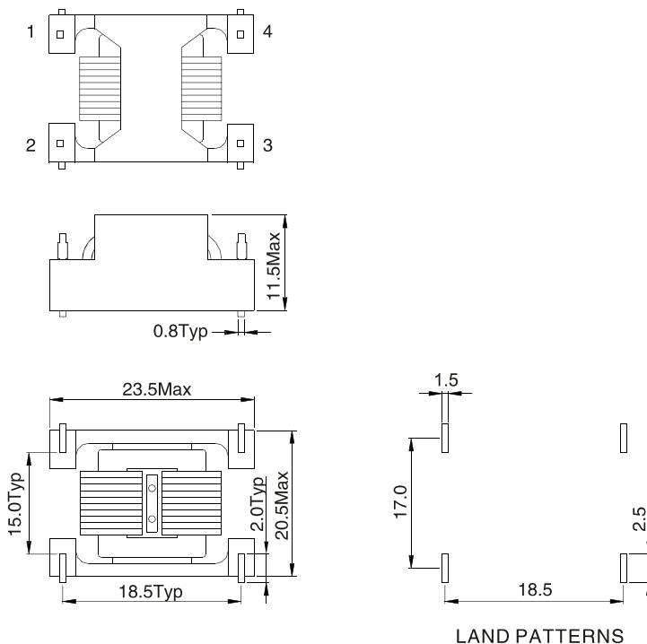
LAND PATTERNS
